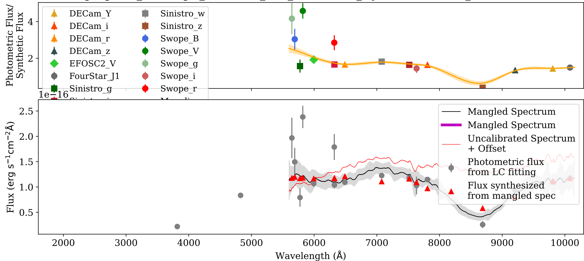
Mangling: VIS_AT2017gfo_ENGRAVE_v1.0_XSHOOTER_MJD-57984.969003_Phase+2.42d.dat
