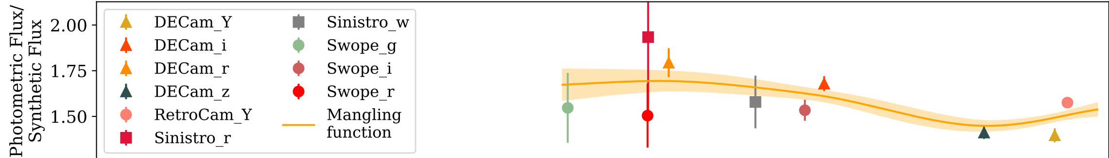
Mangling: VIS_AT2017gfo_ENGRAVE_v1.0_XSHOOTER_MJD-57986.974003_Phase+4.40d.dat
