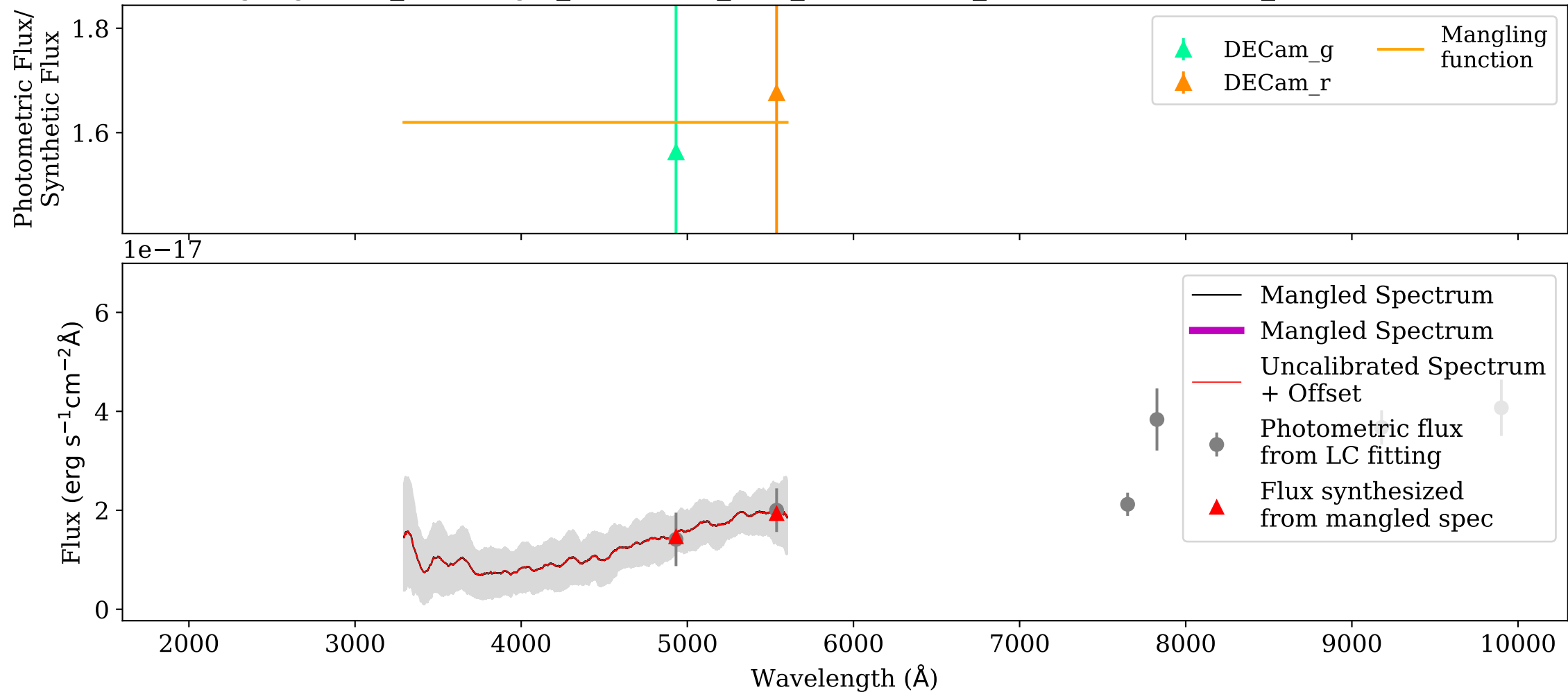
Mangling: UVB_AT2017gfo_ENGRAVE_v1.0_XSHOOTER_MJD-57987.980002_Phase+5.40d.dat
