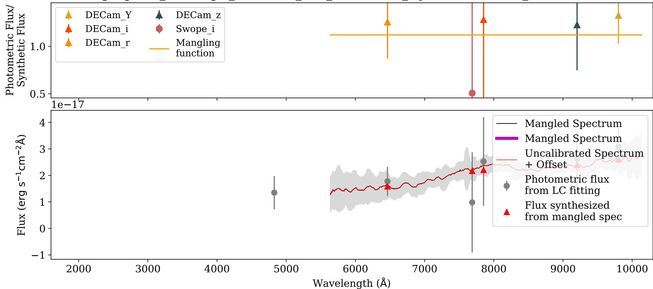
Mangling: VIS_AT2017gfo_ENGRAVE_v1.0_XSHOOTER_MJD-57988.990003_Phase+6.40d.dat
