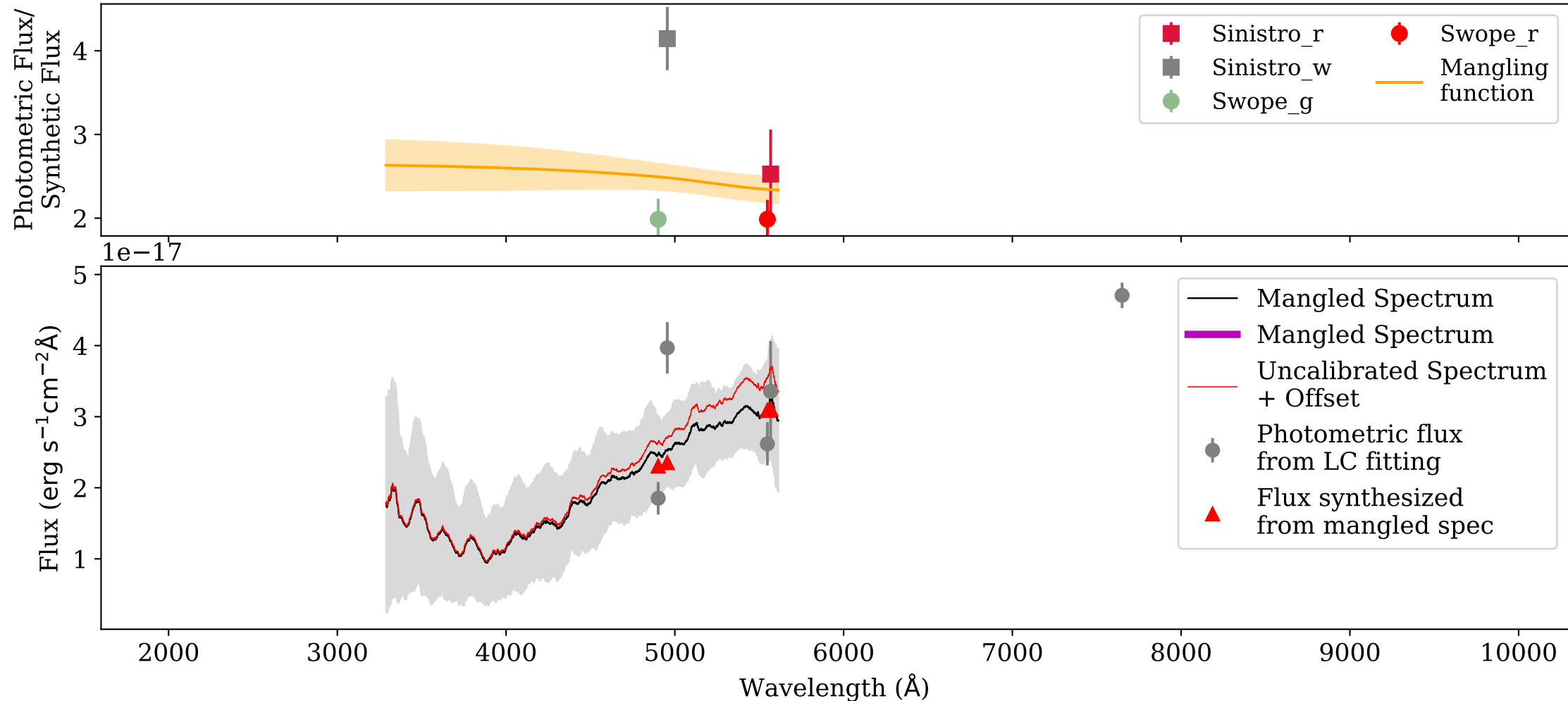
Mangling: UVB_AT2017gfo_ENGRAVE_v1.0_XSHOOTER_MJD-57986.974002_Phase+4.40d.dat
