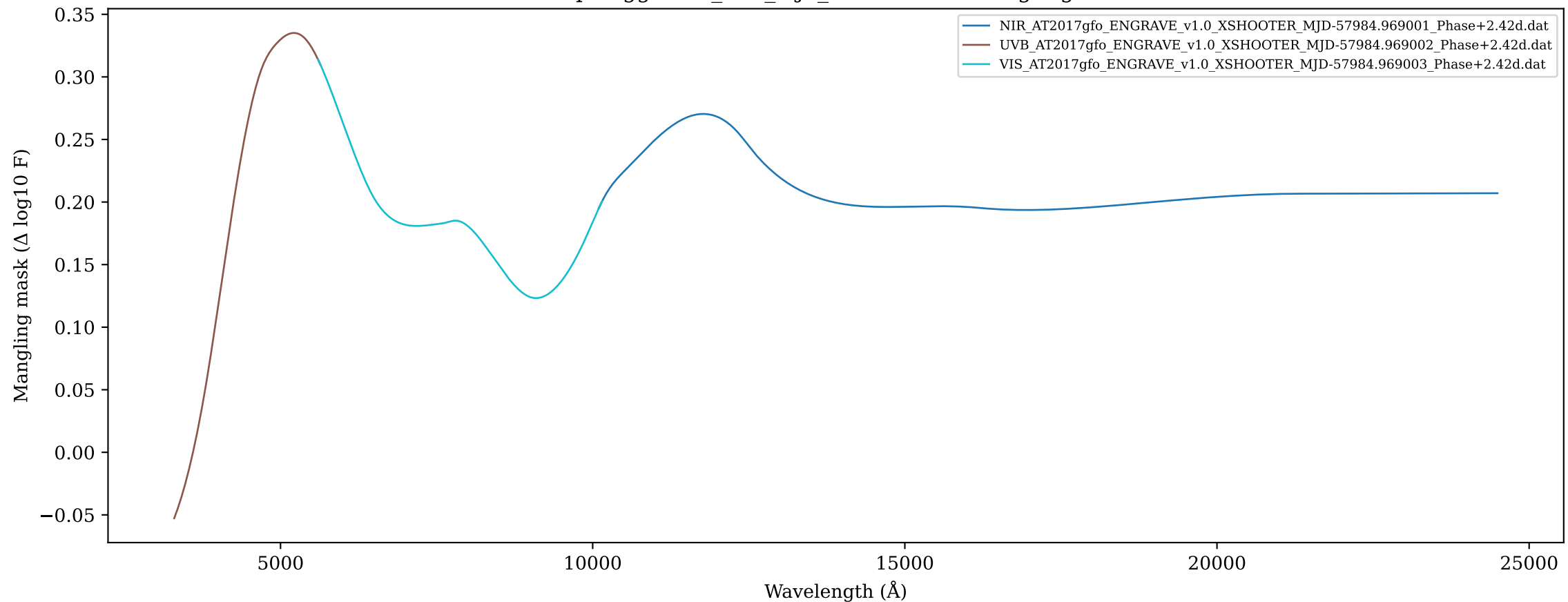
Group suggested_002_mjd_57984.9690 mangling masks
