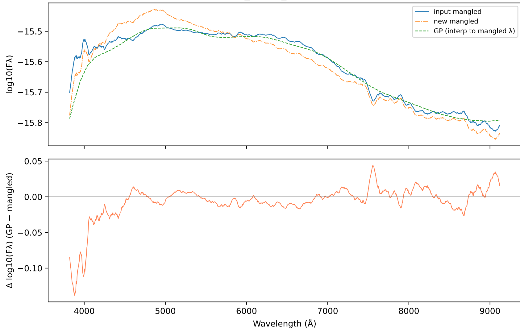
Individual 57983.9914_LDSS3_Magellan.dat MJD 57983.9914
