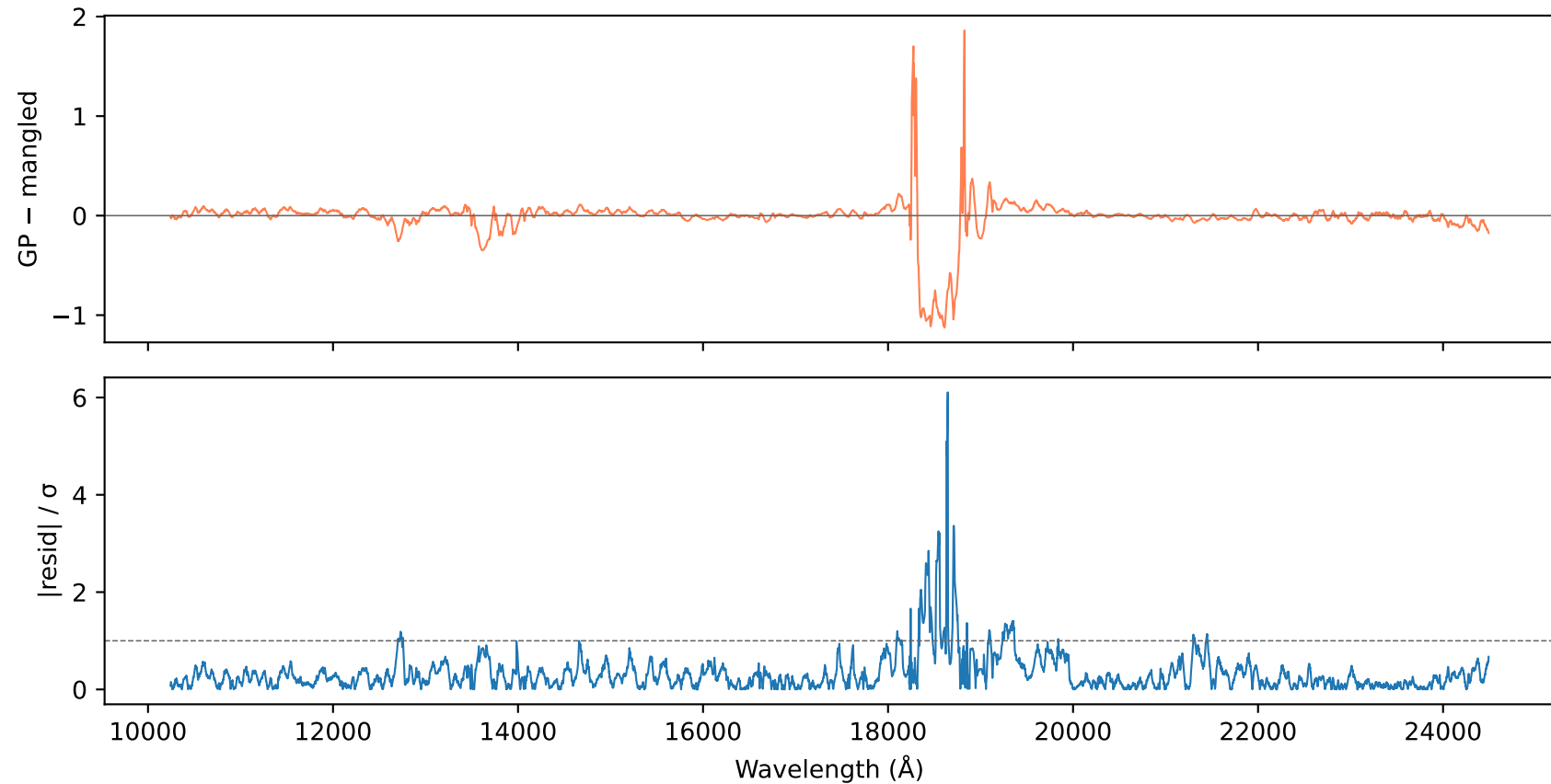
Residuals MJD 57991.0000
