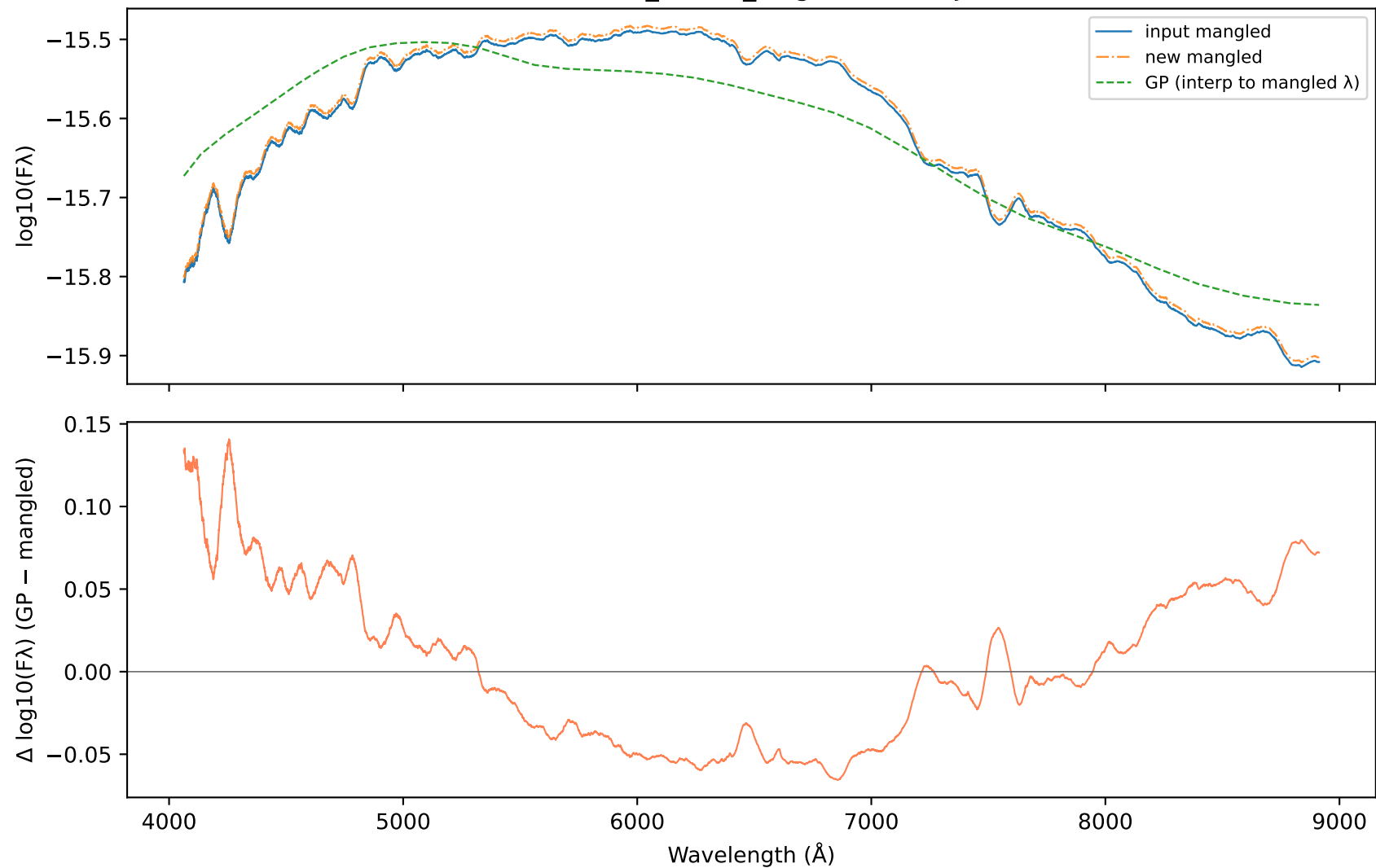
Individual 57984.0484_LDSS3_Magellan.dat MJD 57984.0484
