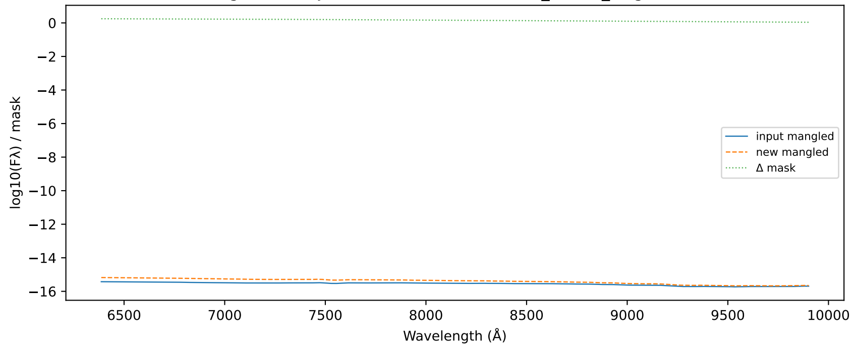
Mangle delta MJD 57983.0362 57983.0362_LDSS3_Magellan.dat
