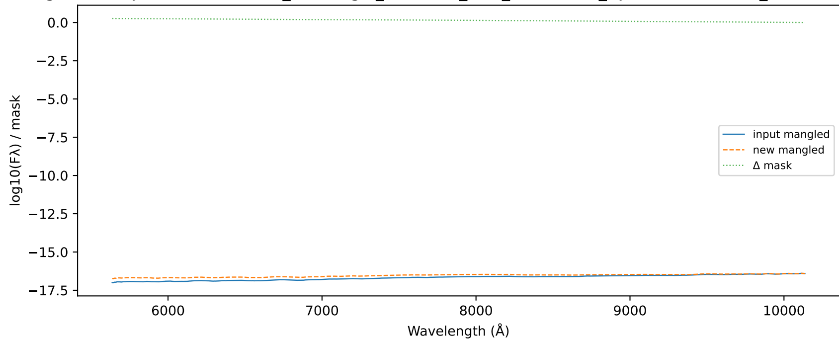
Mangle delta MJD 57988.9900 VIS_AT2017gfo_ENGRAVE_v1.0_XSHOOTER_MJD-57988.990003_Phase+6.40d.dat
