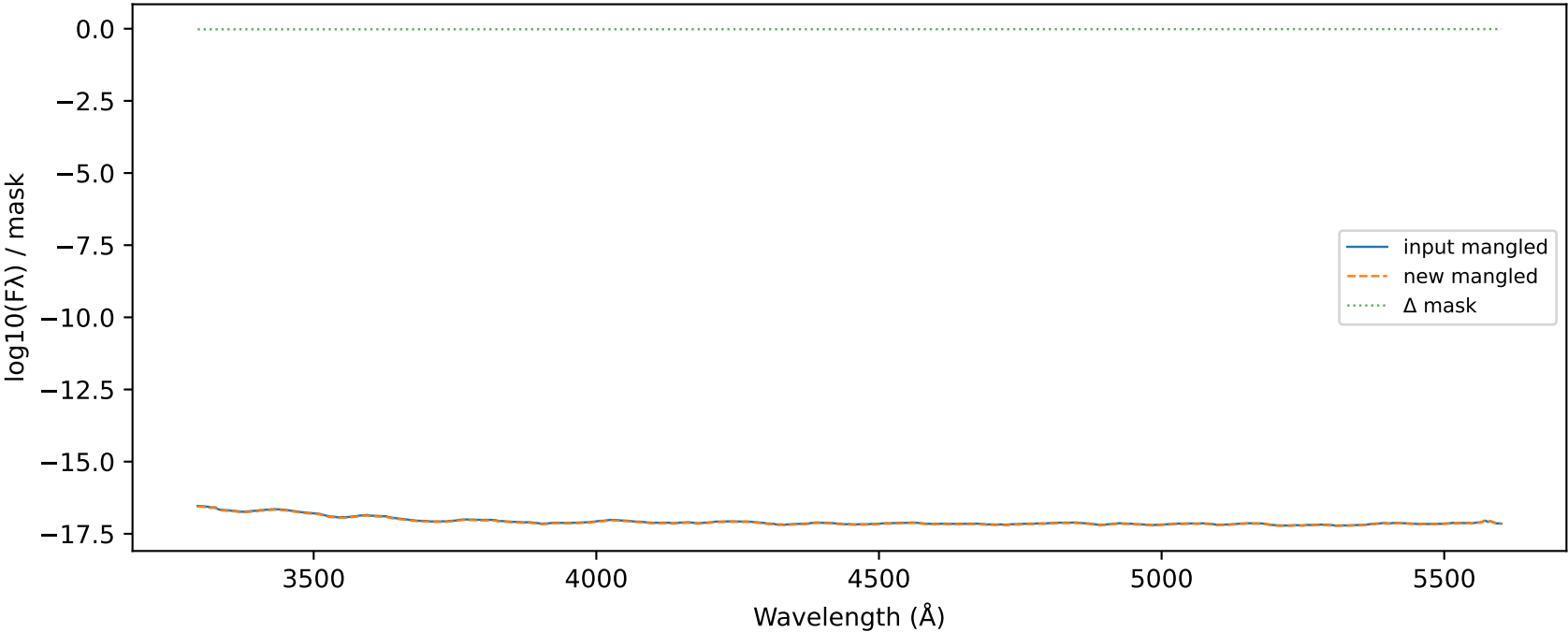
Mangle delta MJD 57992.0000 UVB_AT2017gfo_ENGRAVE_v1.0_XSHOOTER_MJD-57992.000002_Phase+9.40d.dat
