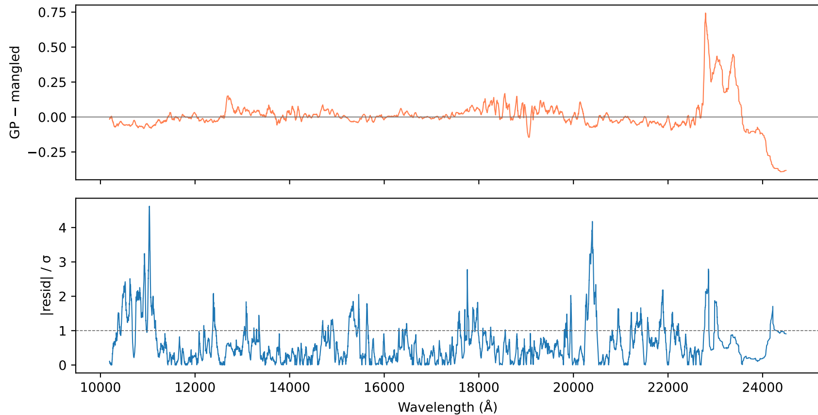
Residuals MJD 57986.9740
