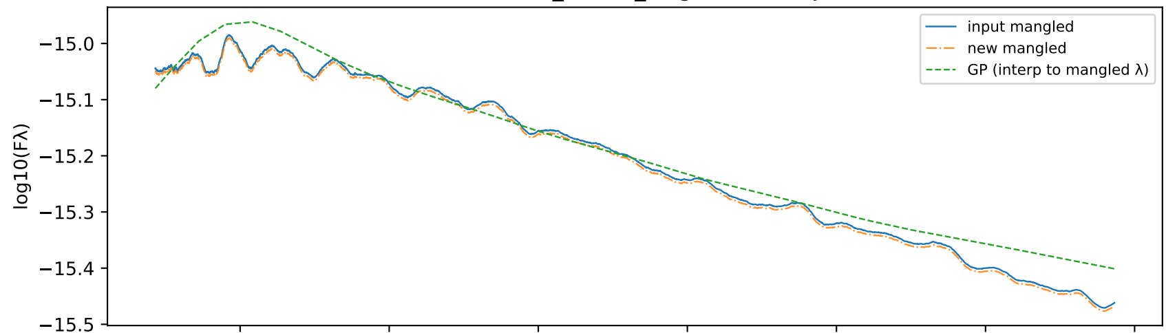
Individual 57983.05998_LDSS3_Magellan.dat MJD 57983.0600
