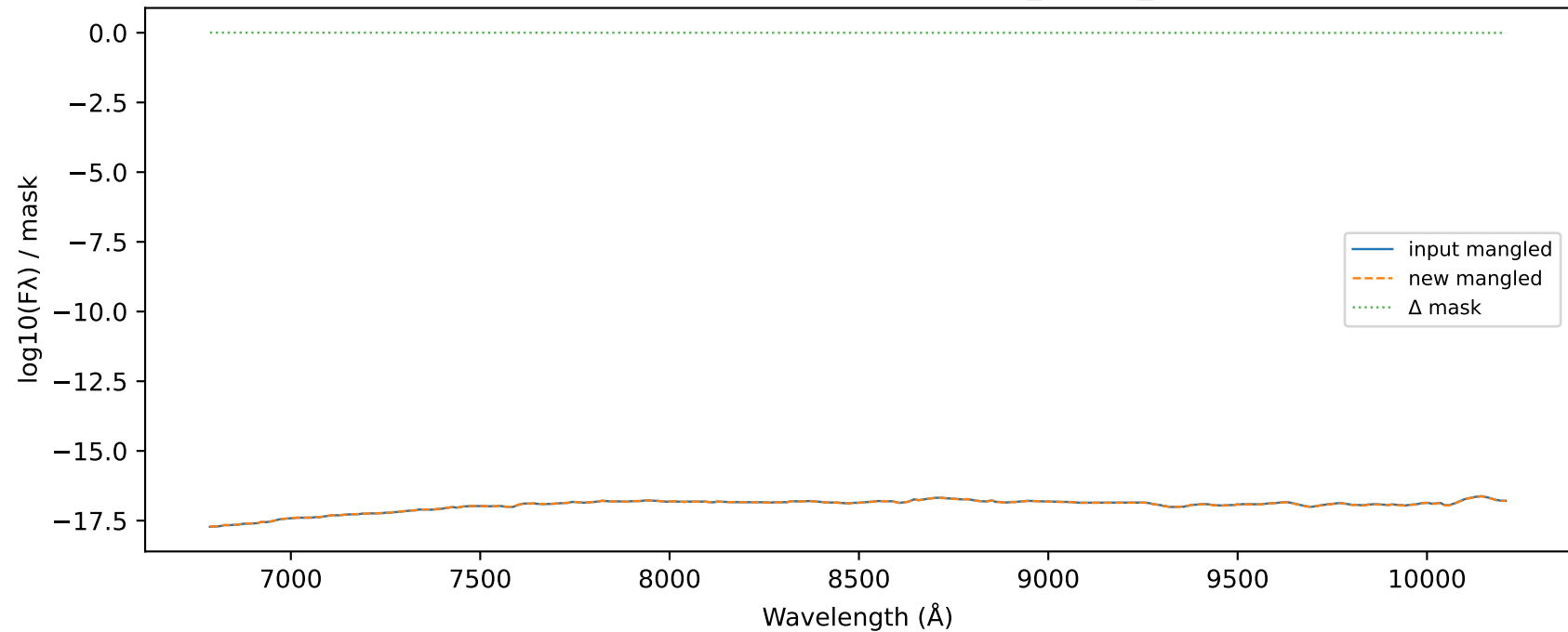
Mangle delta MJD 57990.9856 57990.98563_LDSS3_Magellan.dat
