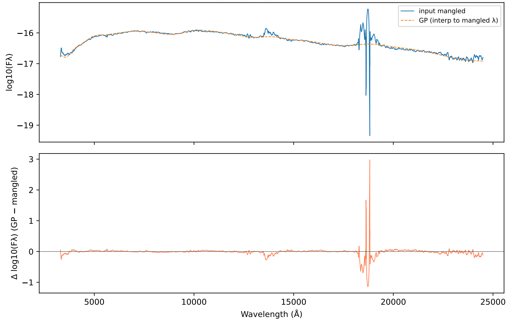
Group suggested_002_mjd_57984.9690 MJD 57984.9690
