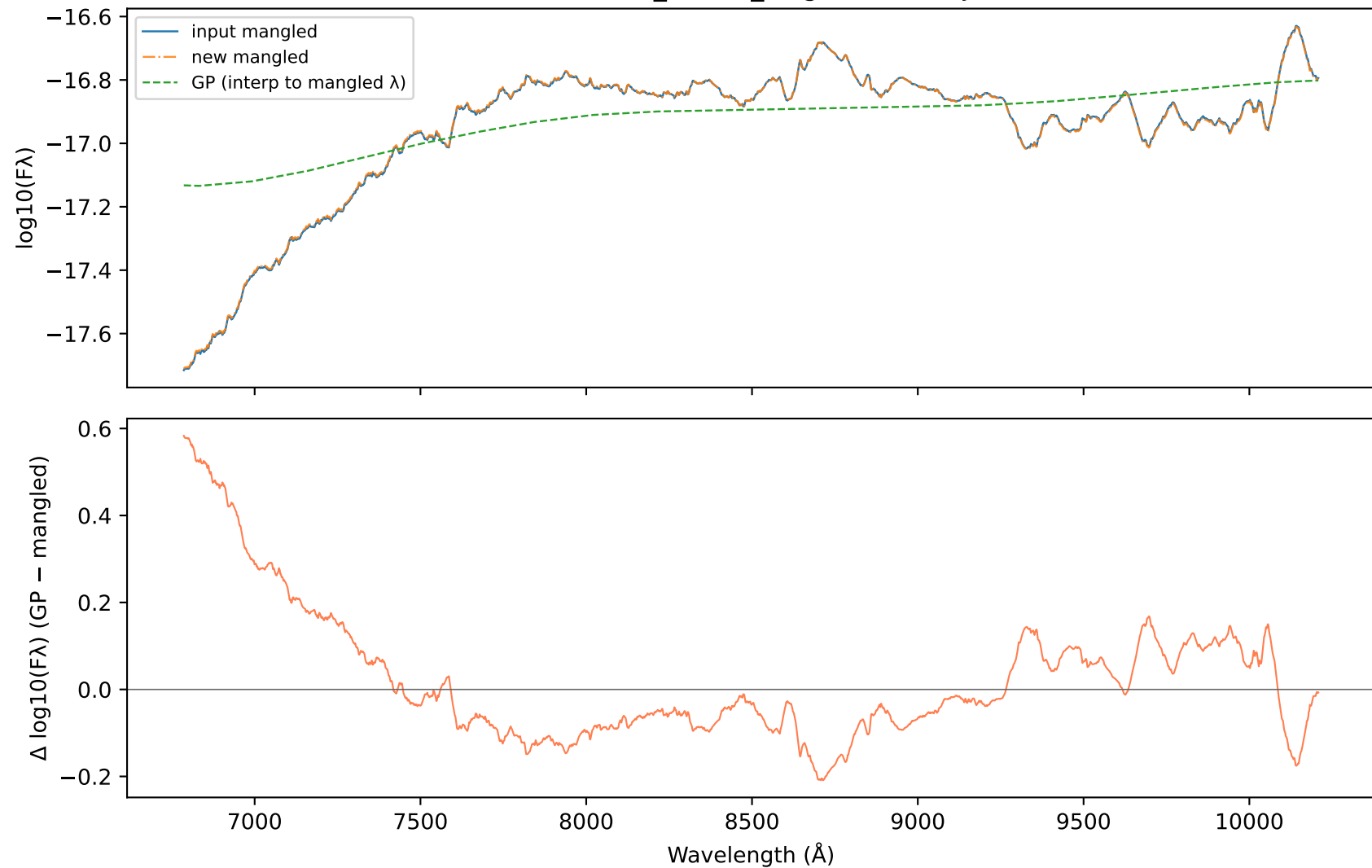
Individual 57990.98563_LDSS3_Magellan.dat MJD 57990.9856
