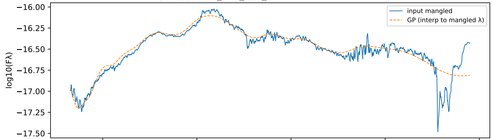
Group suggested_004_mjd_57986.9740 MJD 57986.9740
