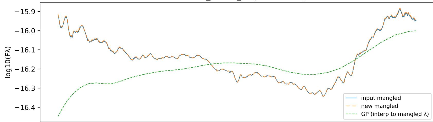
Individual 57985.99019_LDSS3_Magellan.dat MJD 57985.9902
