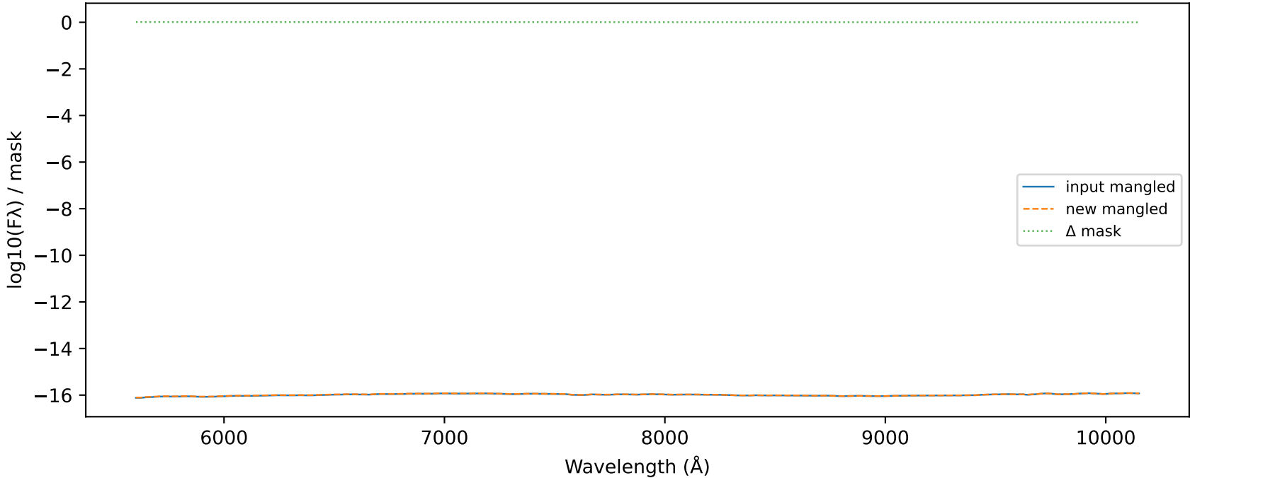
Mangle delta MJD 57984.9690 VIS_AT2017gfo_ENGRAVE_v1.0_XSHOOTER_MJD-57984.969003_Phase+2.42d.dat
