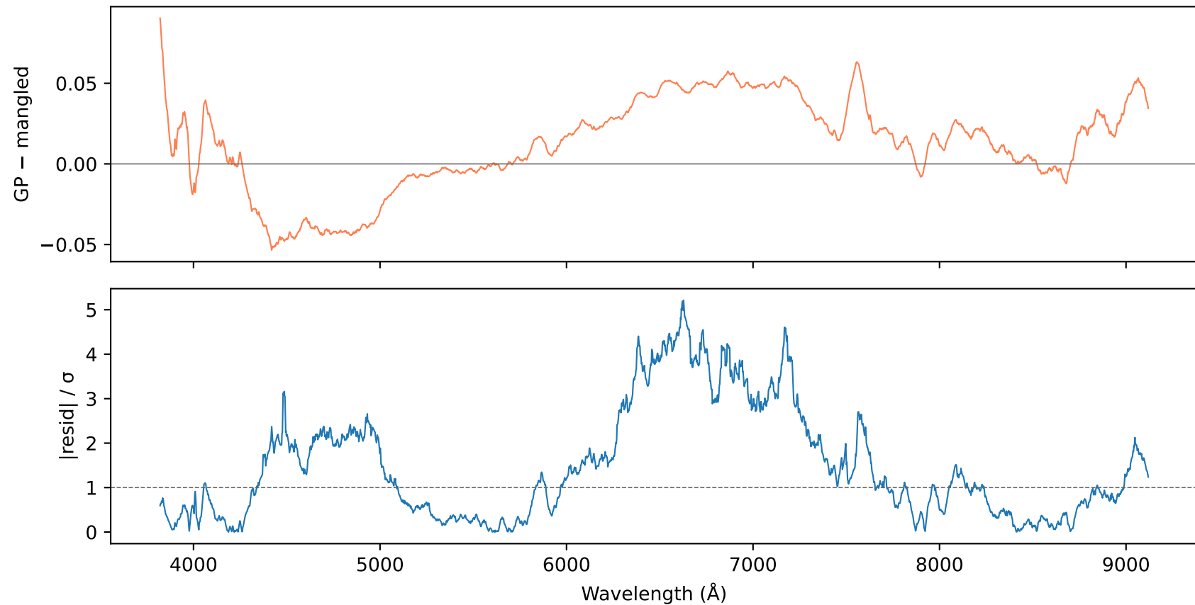
Residuals MJD 57983.9914
