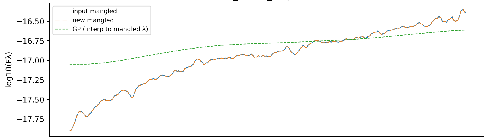
Individual 57989.98185_LDSS3_Magellan.dat MJD 57989.9818
