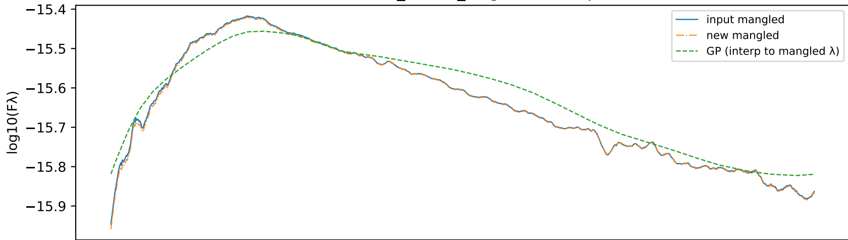
Individual 57983.9914_LDSS3_Magellan.dat MJD 57983.9914
