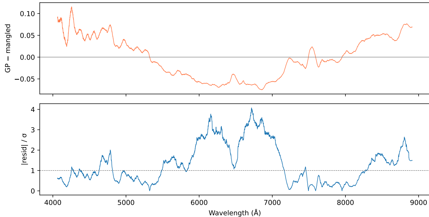
Residuals MJD 57984.0484
