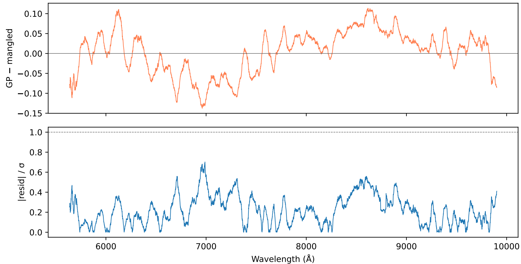
Residuals MJD 57993.0000
