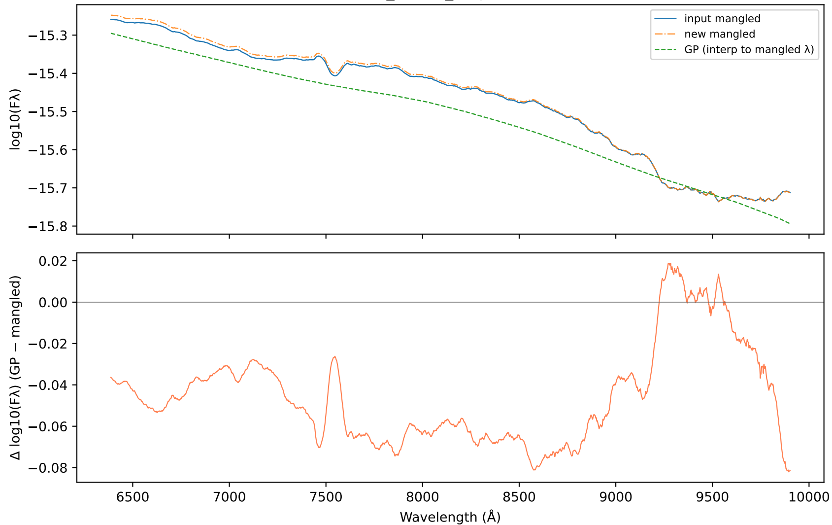
Individual 57983.0362_LDSS3_Magellan.dat MJD 57983.0362
