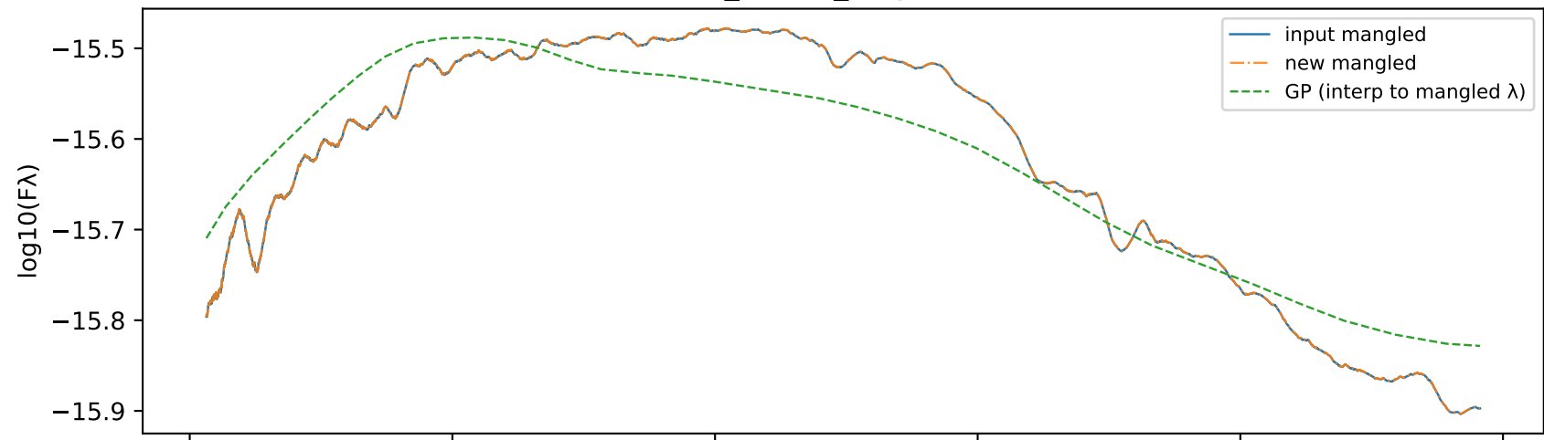
Individual 57984.0484_LDSS3_Magellan.dat MJD 57984.0484
