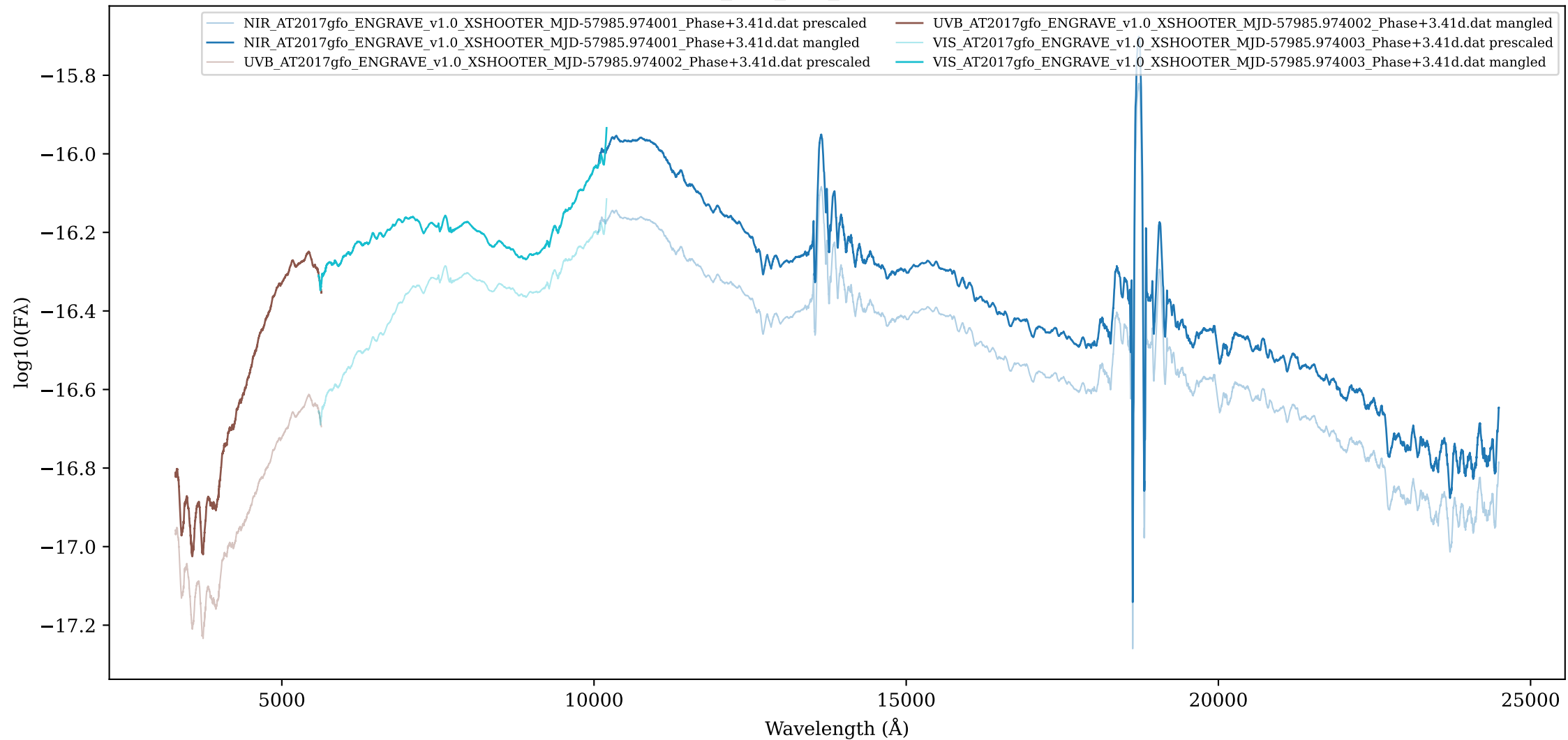
Mangle group suggested_003_mjd_57985.9740: prescaled vs mangled
