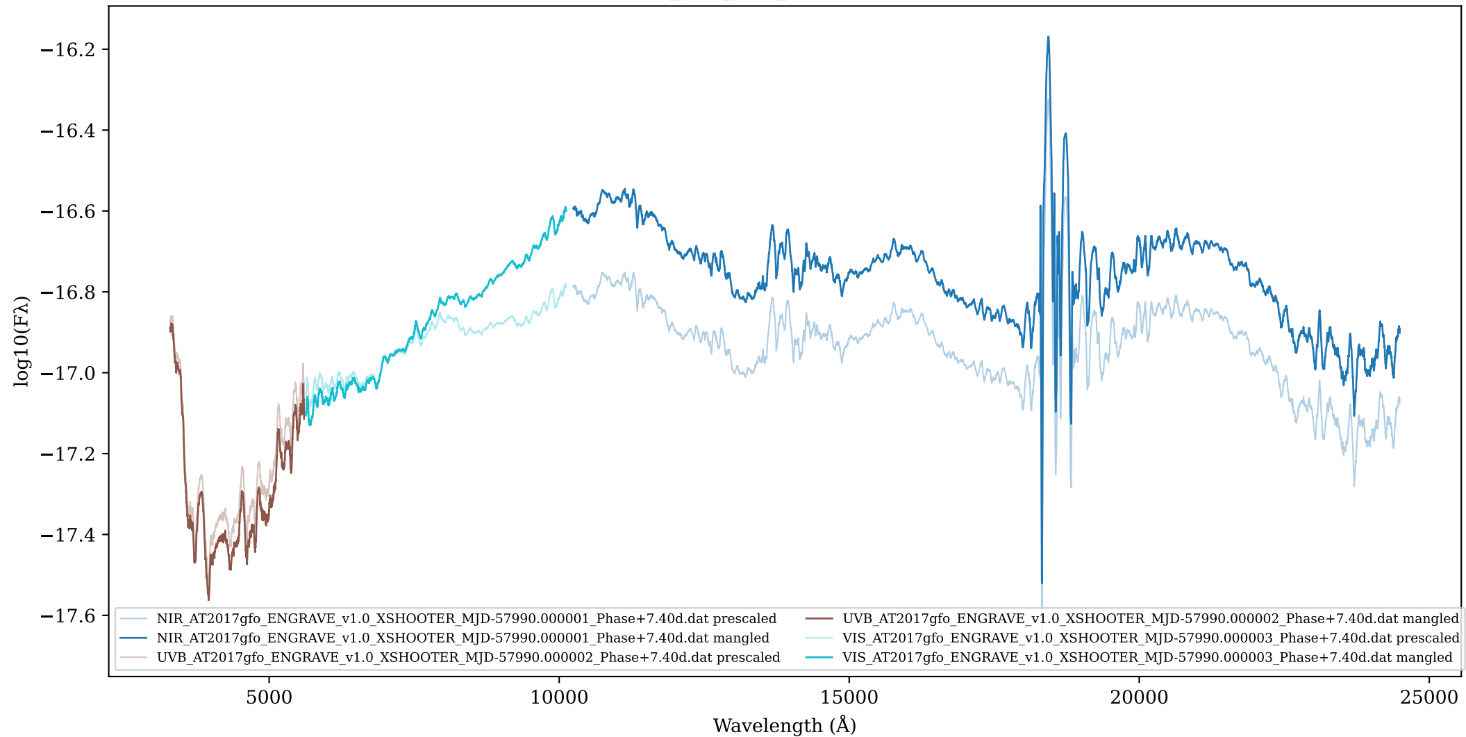
Mangle group suggested_007_mjd_57990.0000: prescaled vs mangled
