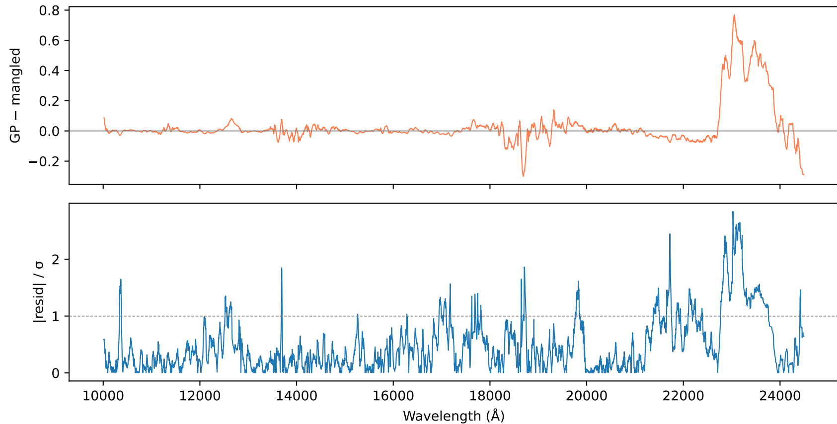
Residuals MJD 57983.9690
