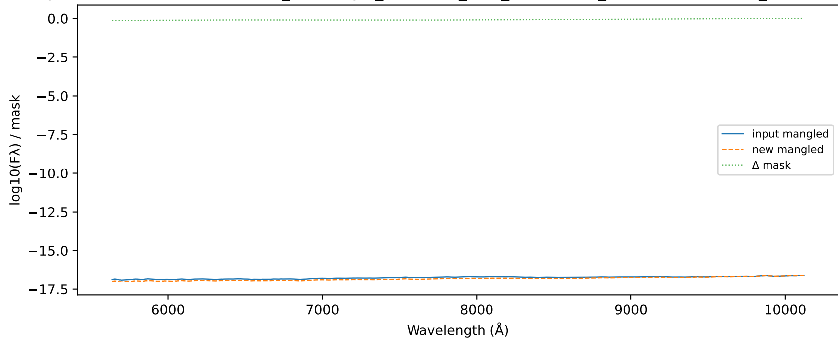
Mangle delta MJD 57990.0000 VIS_AT2017gfo_ENGRAVE_v1.0_XSHOOTER_MJD-57990.000003_Phase+7.40d.dat
