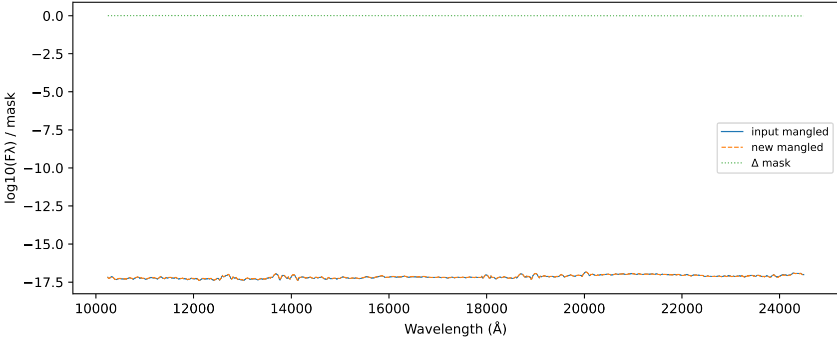
Mangle delta MJD 57993.0000 NIR_AT2017gfo_ENGRAVE_v1.0_XSHOOTER_MJD-57993.000001_Phase+10.40d.dat
