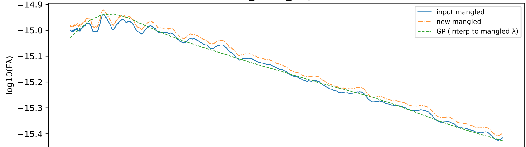
Individual 57983.05998_LDSS3_Magellan.dat MJD 57983.0600
