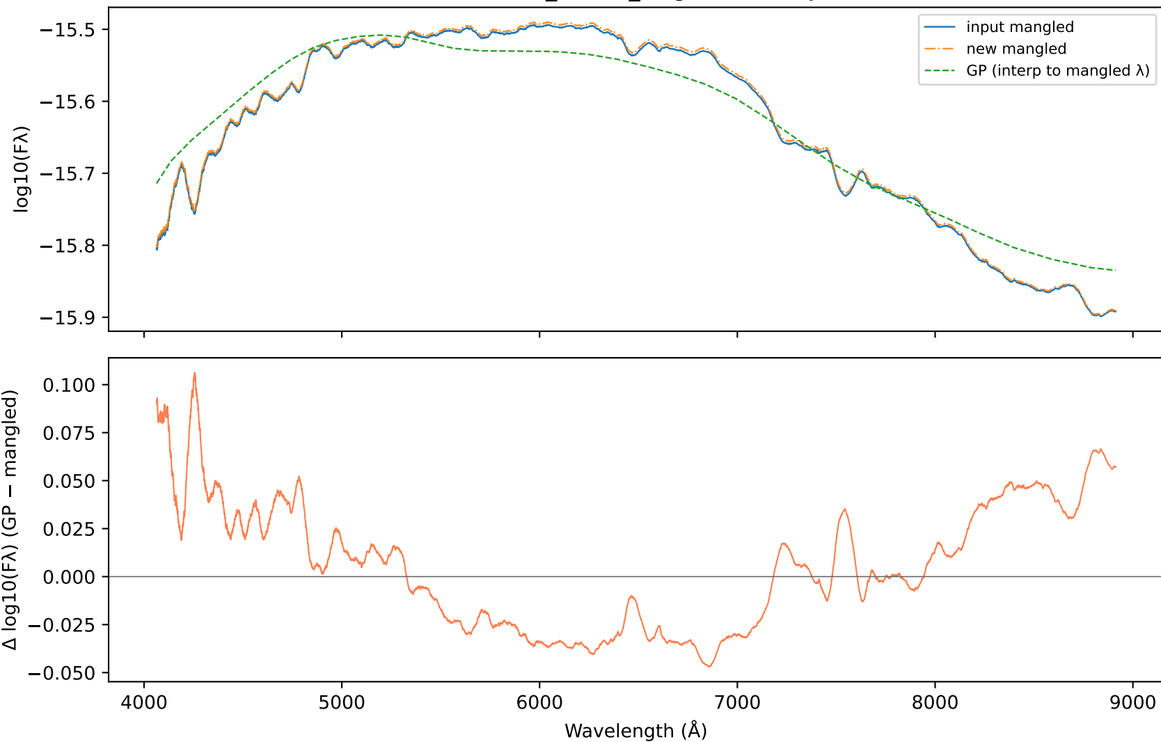
Individual 57984.0484_LDSS3_Magellan.dat MJD 57984.0484
