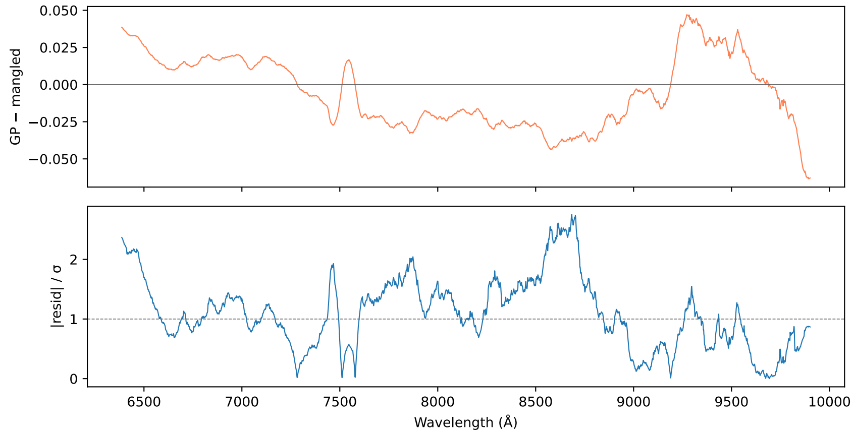
Residuals MJD 57983.0362
