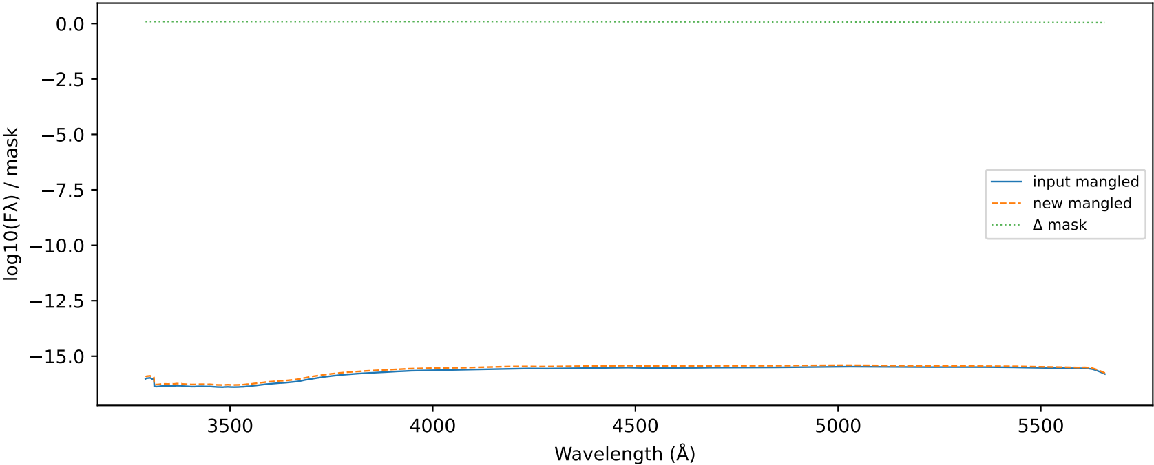
Mangle delta MJD 57983.9690 UVB_AT2017gfo_ENGRAVE_v1.0_XSHOOTER_MJD-57983.969002_Phase+1.43d.dat
