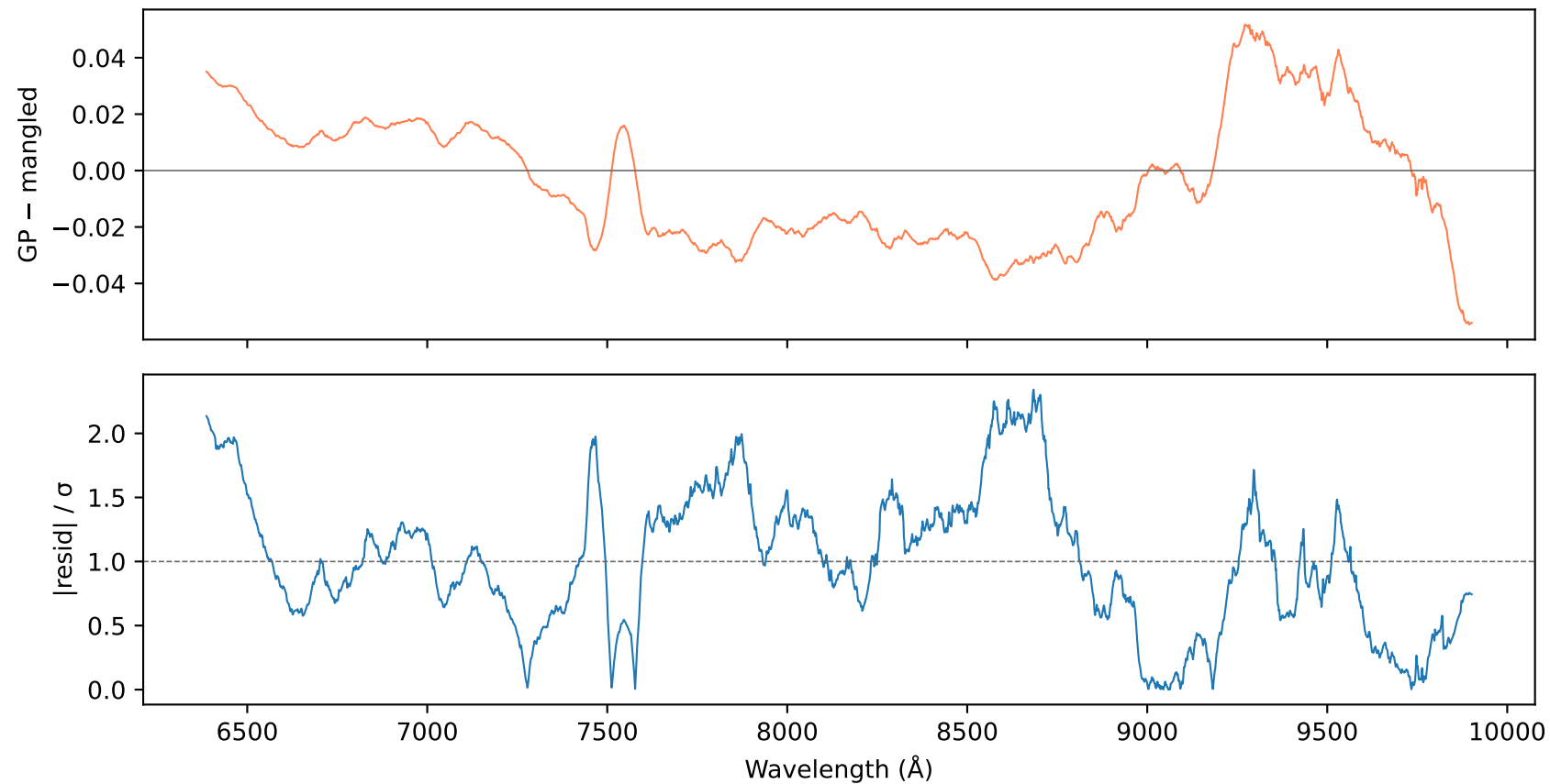
Residuals MJD 57983.0362
