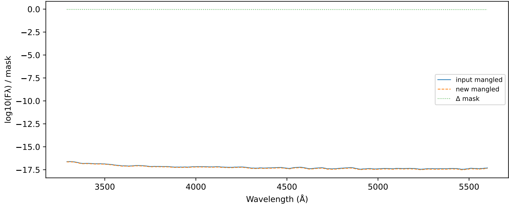
Mangle delta MJD 57993.0000 UVB_AT2017gfo_ENGRAVE_v1.0_XSHOOTER_MJD-57993.000002_Phase+10.40d.dat
