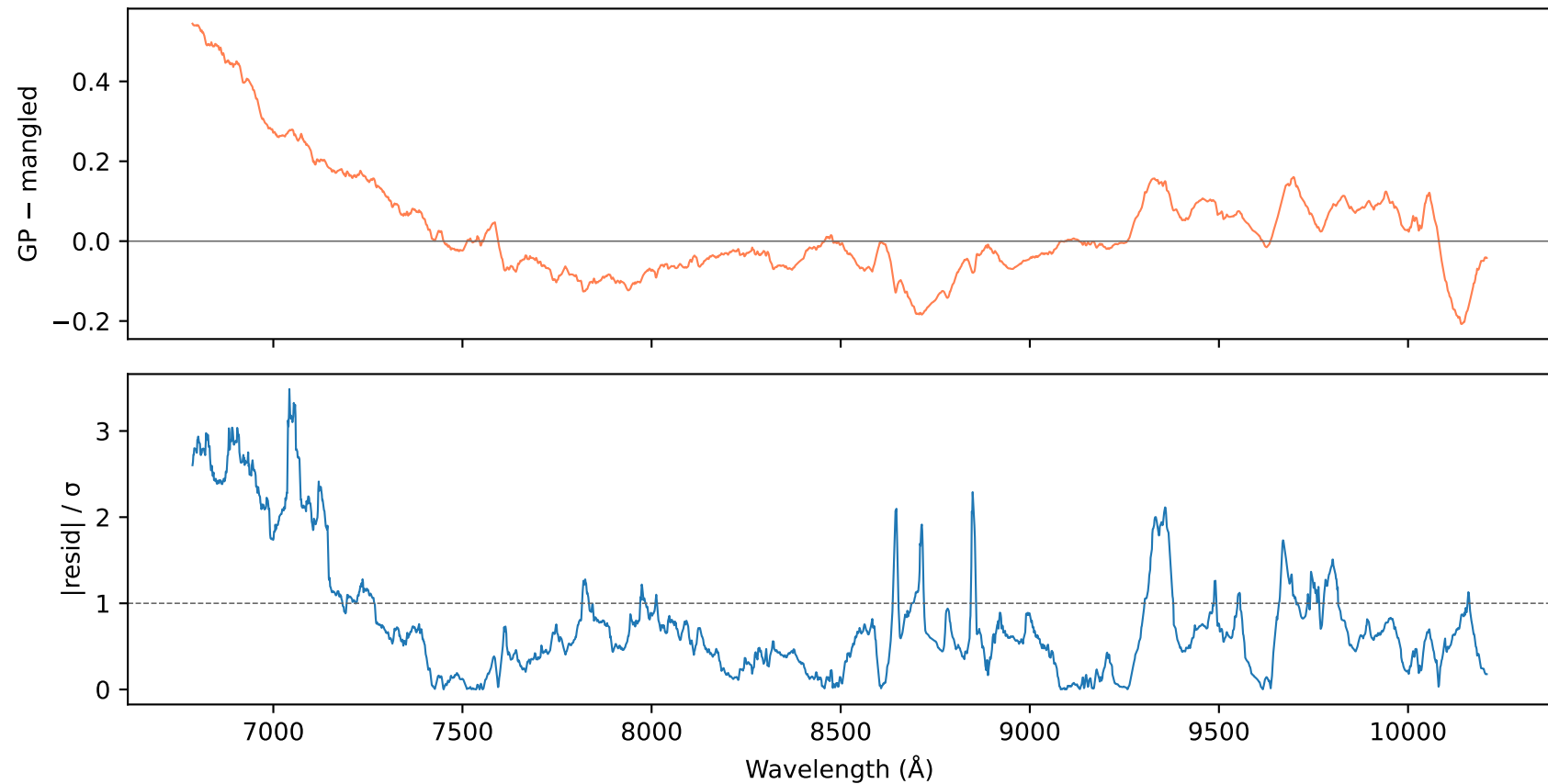
Residuals MJD 57990.9856
