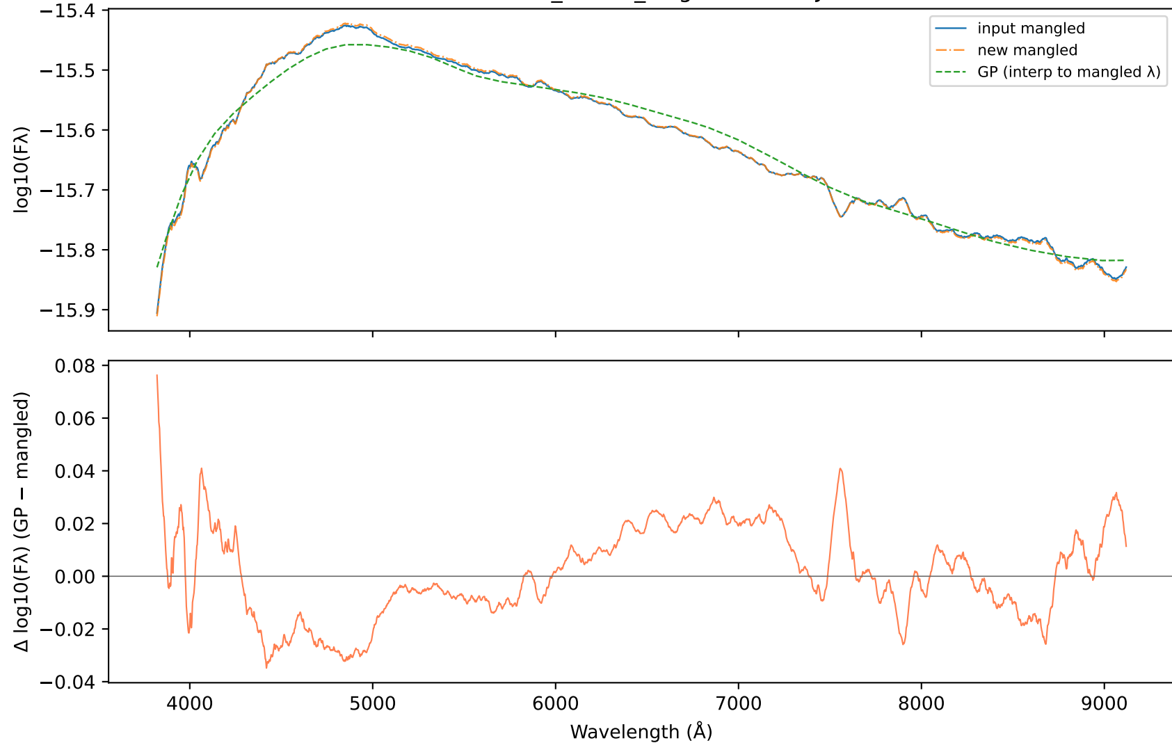
Individual 57983.9914_LDSS3_Magellan.dat MJD 57983.9914
