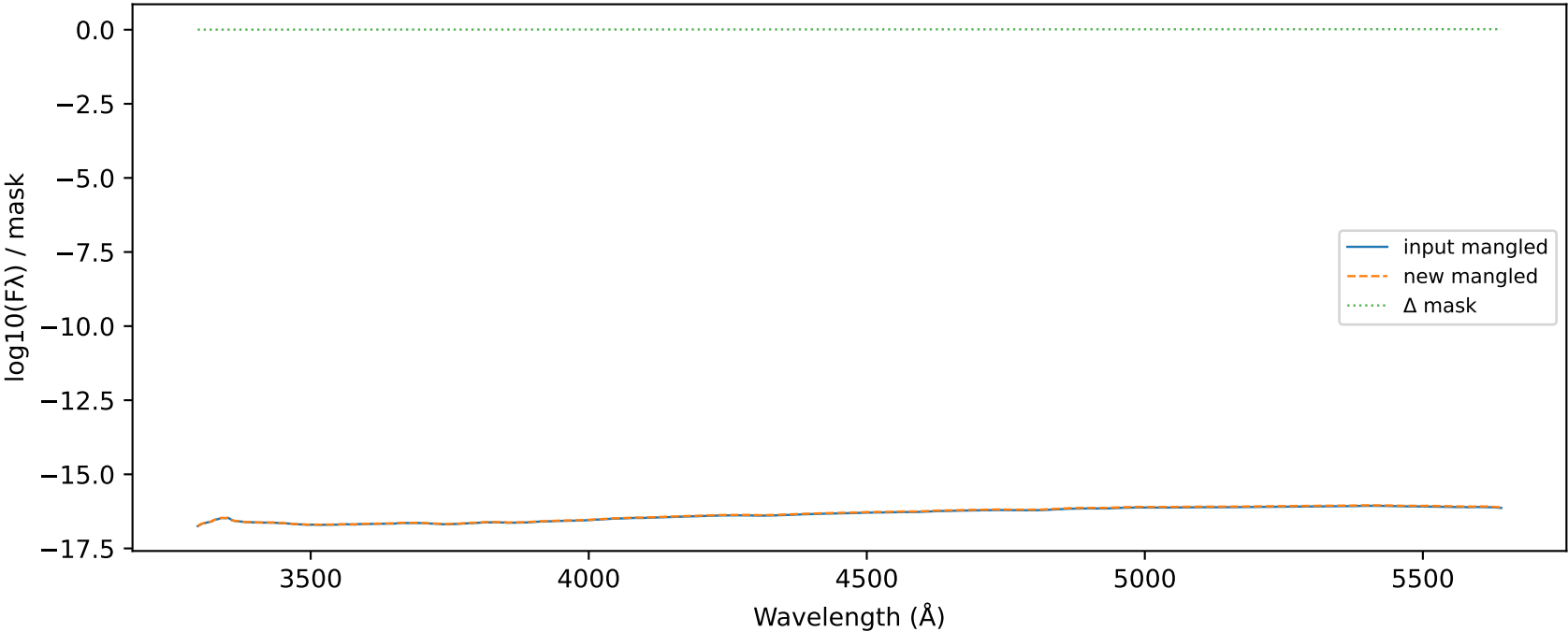
Mangle delta MJD 57984.9690 UVB_AT2017gfo_ENGRAVE_v1.0_XSHOOTER_MJD-57984.969002_Phase+2.42d.dat
