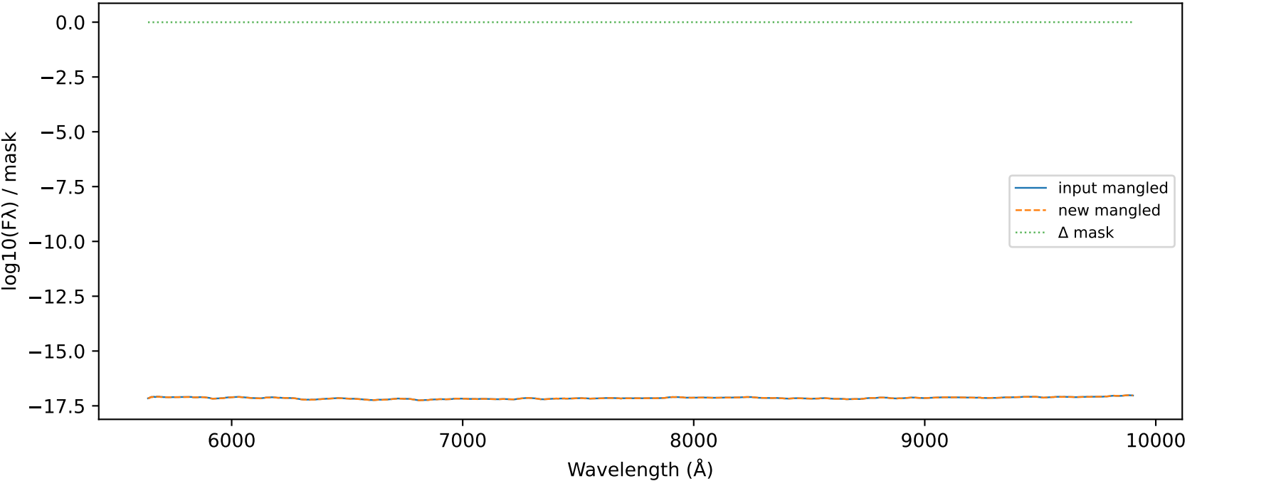
Mangle delta MJD 57992.0000 VIS_AT2017gfo_ENGRAVE_v1.0_XSHOOTER_MJD-57992.000003_Phase+9.40d.dat
