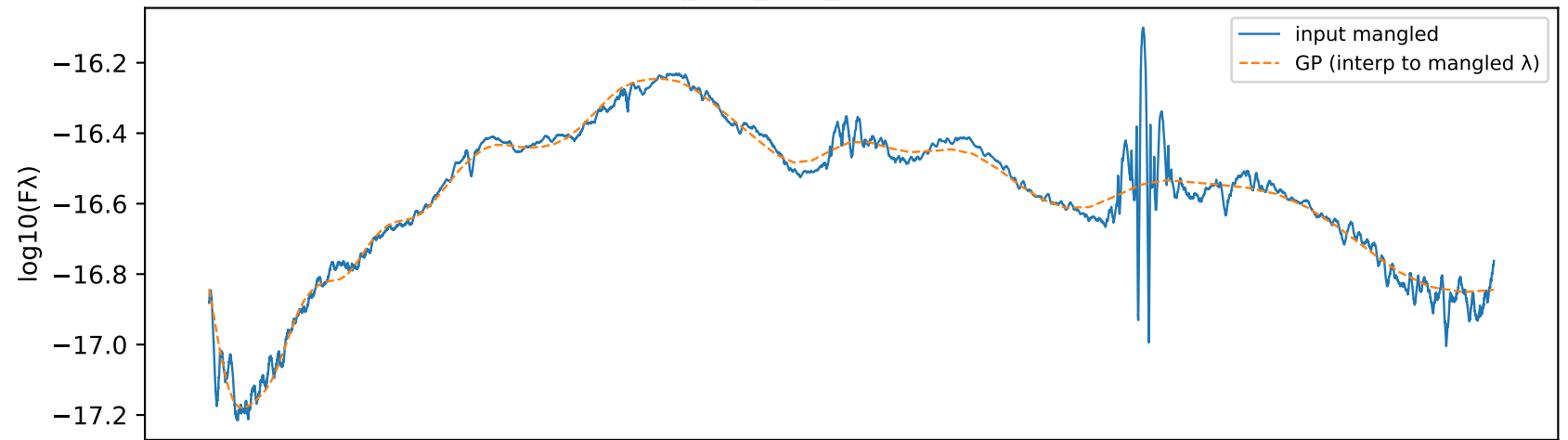
Group suggested_005_mjd_57987.9800 MJD 57987.9800
