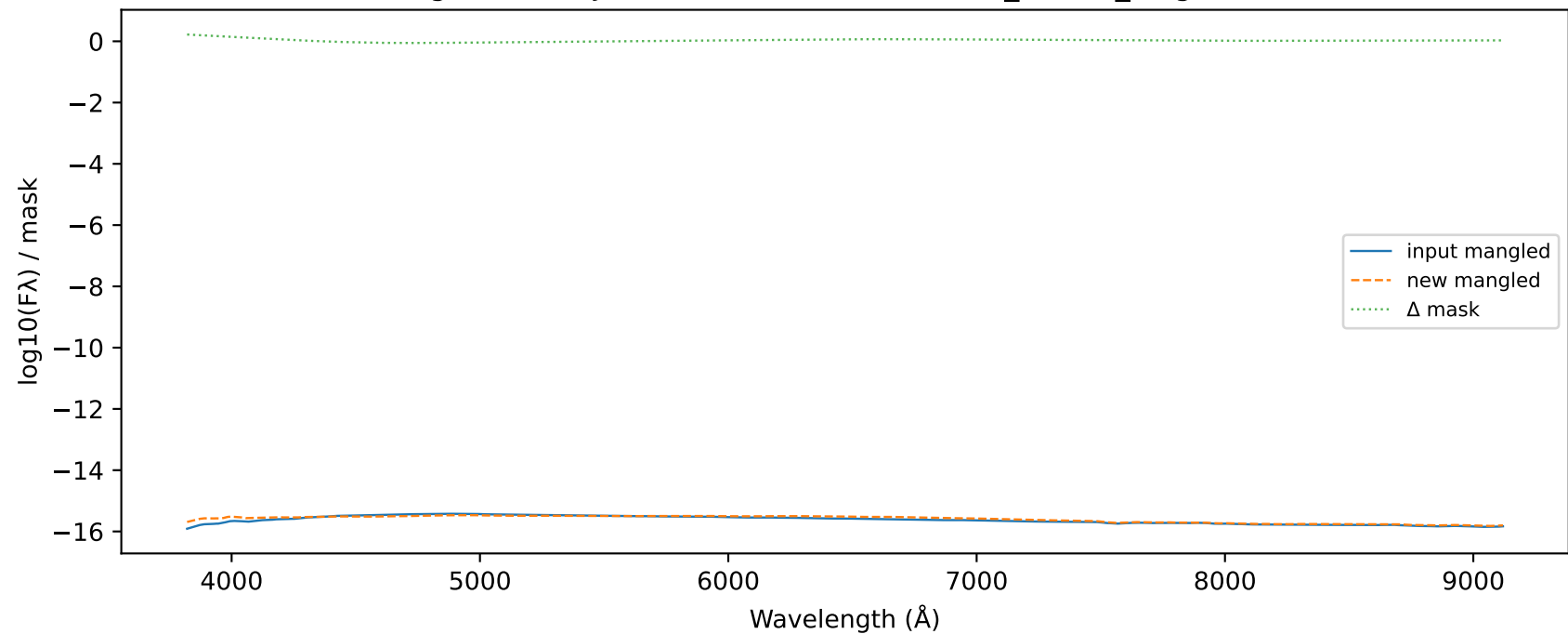
Mangle delta MJD 57983.9914 57983.9914_LDSS3_Magellan.dat
