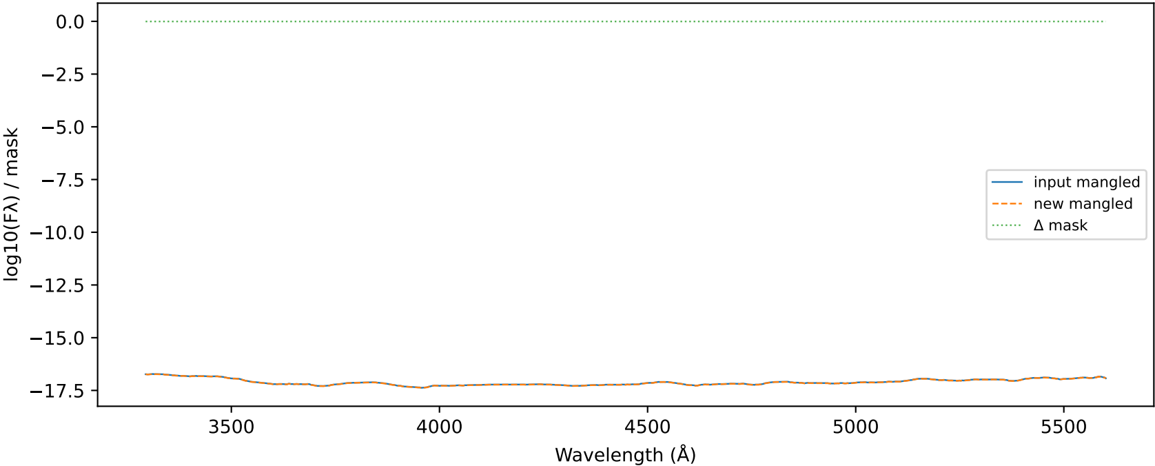
Mangle delta MJD 57990.0000 UVB_AT2017gfo_ENGRAVE_v1.0_XSHOOTER_MJD-57990.000002_Phase+7.40d.dat
