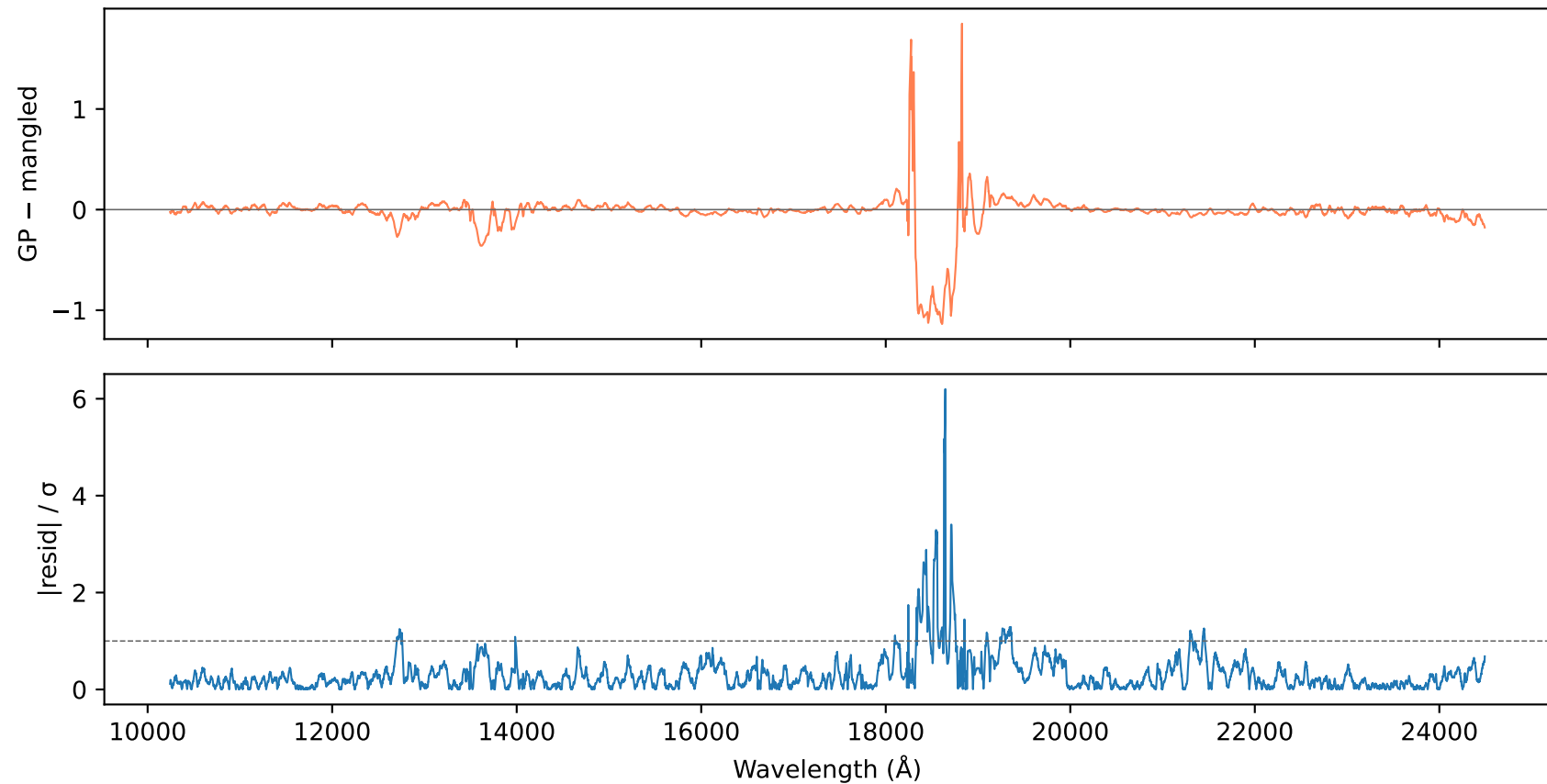
Residuals MJD 57991.0000
