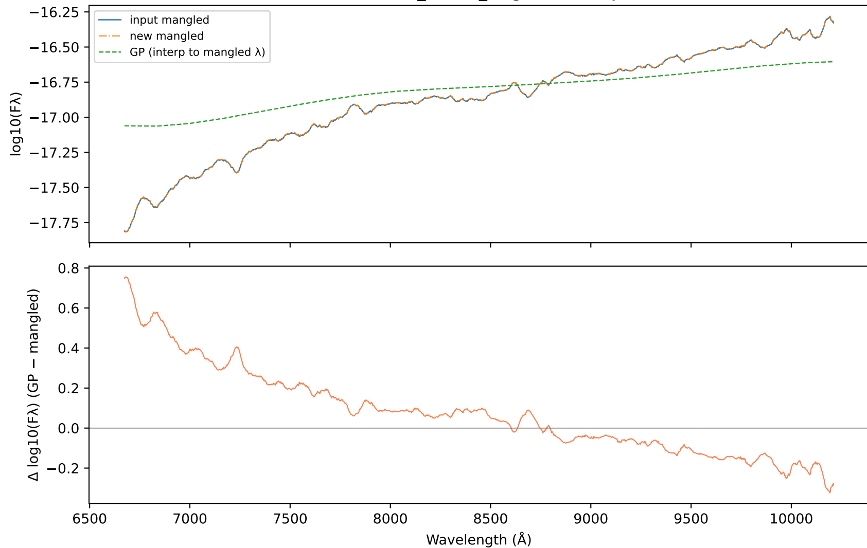
Individual 57989.98185_LDSS3_Magellan.dat MJD 57989.9818
