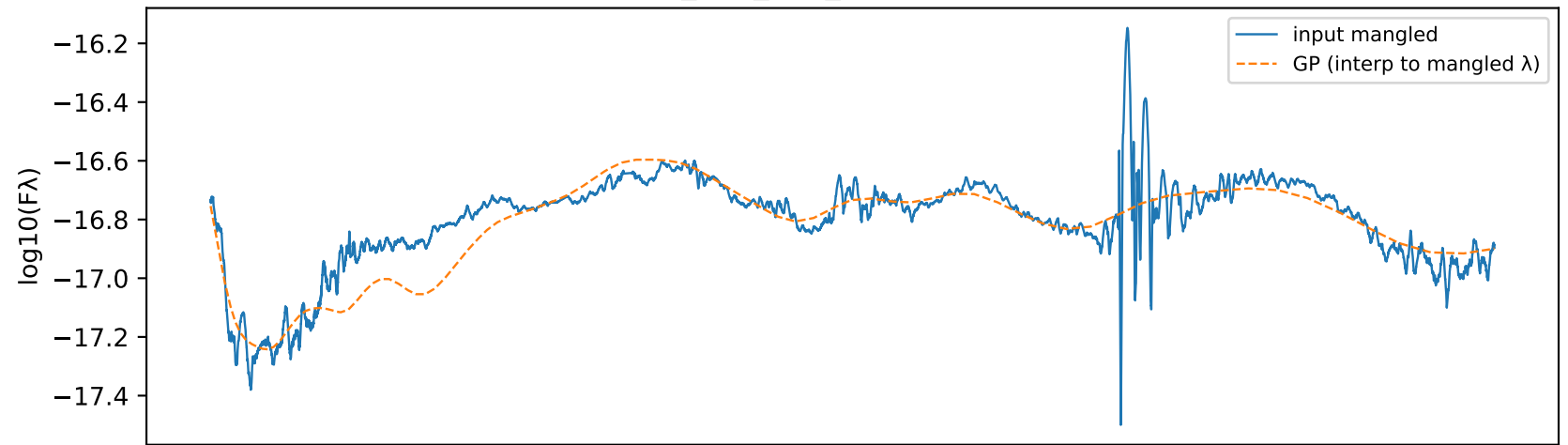
Group suggested_007_mjd_57990.0000 MJD 57990.0000
