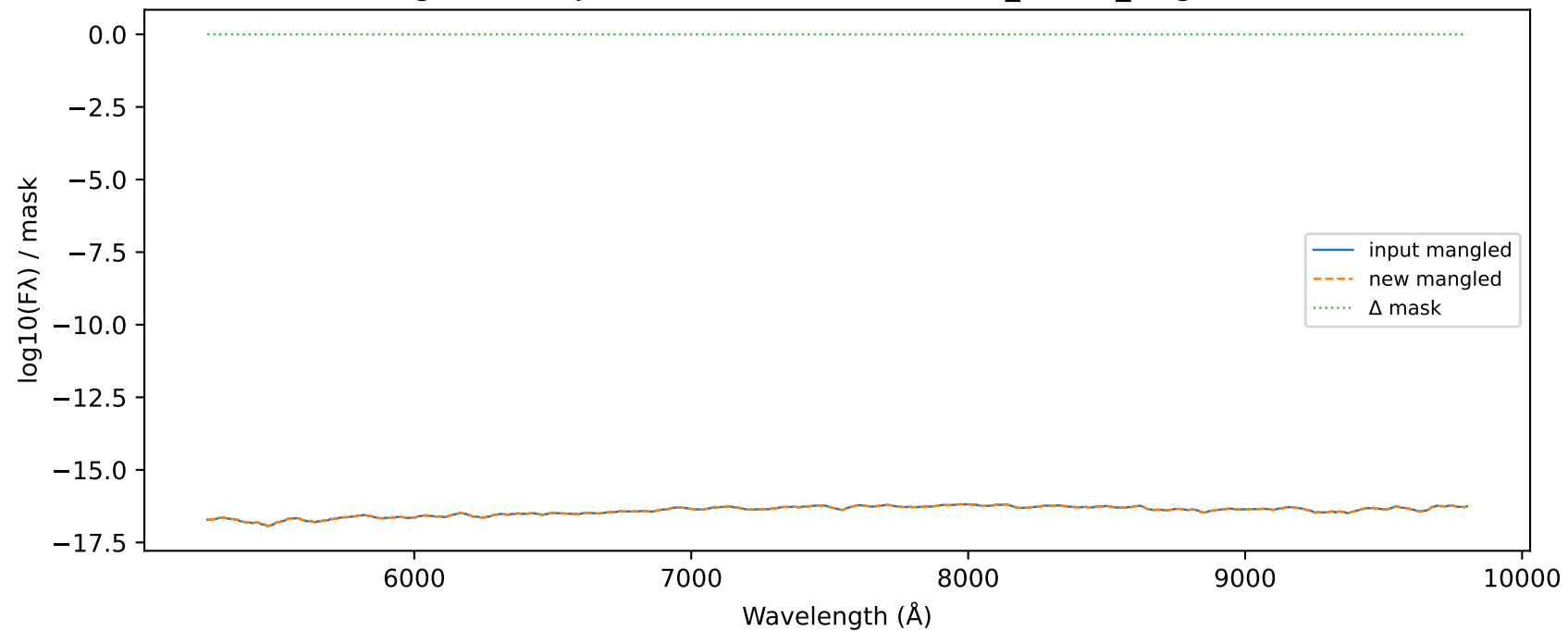
Mangle delta MJD 57987.0351 57987.03511_LDSS3_Magellan.dat
