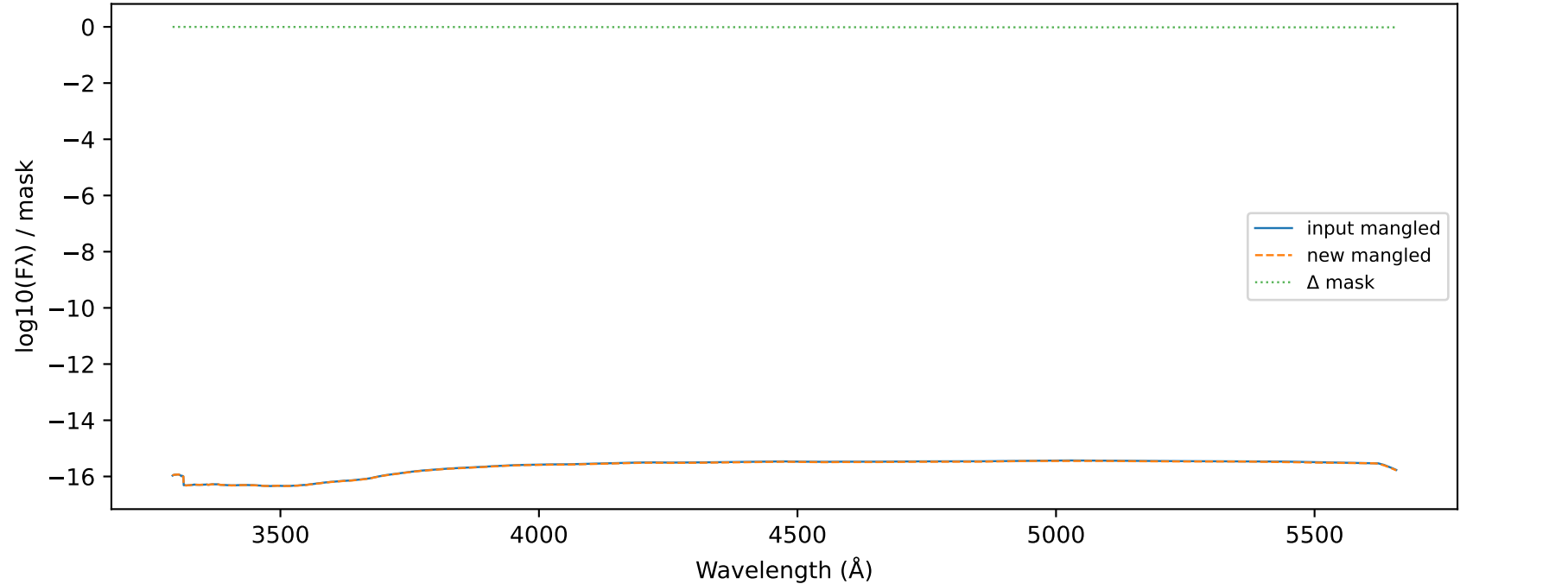
Mangle delta MJD 57983.9690 UVB_AT2017gfo_ENGRAVE_v1.0_XSHOOTER_MJD-57983.969002_Phase+1.43d.dat
